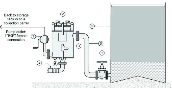
Fig 2: Installation including Manual Pump with elevation spool
